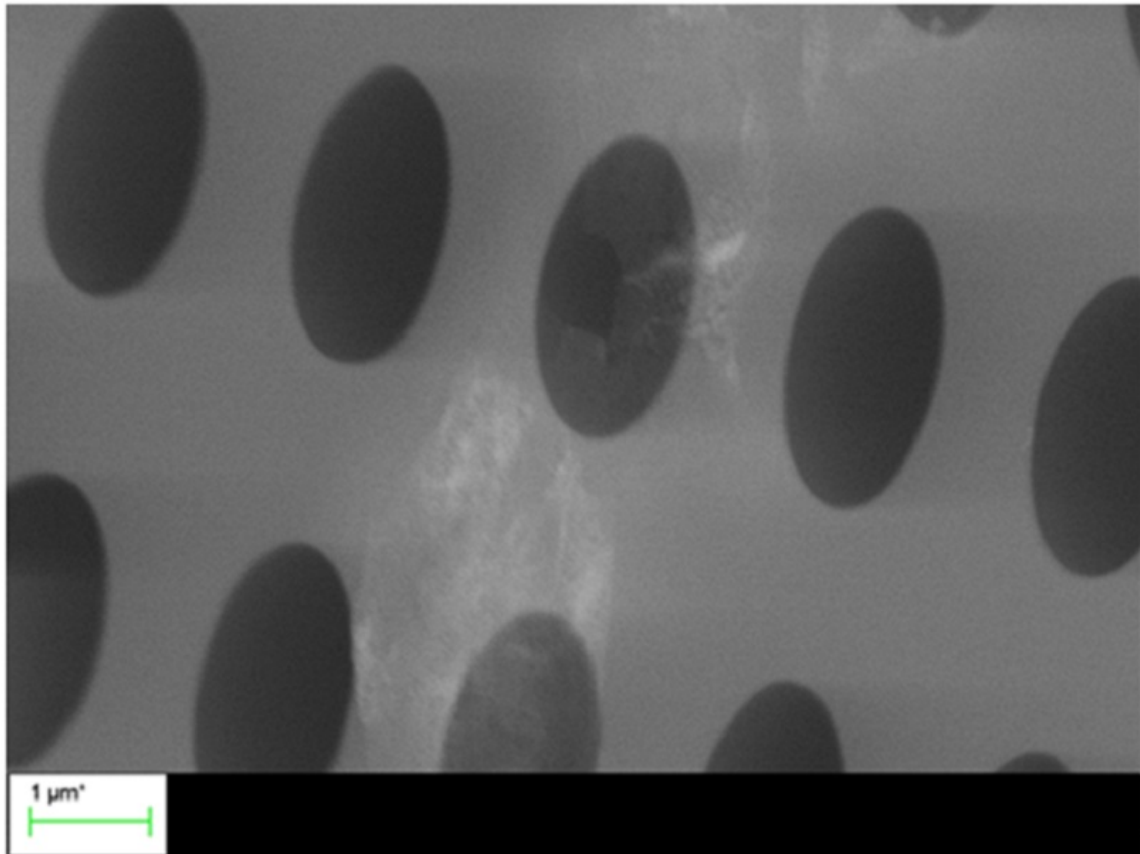
Figure 2: Scanning electron microscopy image of a graphene membrane transferred on a Si3N4 [Courtesy of Professor Sergey Kubatkin, Chalmers University]
